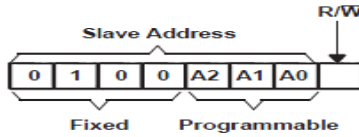
Address Reference
